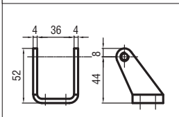
Galvanized steel sliding bracket part No. 40235F. It allows the fixing for the whole length of the actuator. To use only for single Rack.
