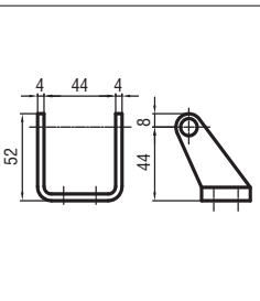
Galvanized steel sliding bracket part No. 40235F. It allows the fixing for the whole length of the actuator. To use only for single Rack.
